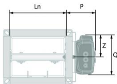
An < 400mm
